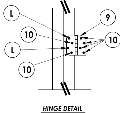
HINGE DETAIL
