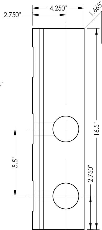
4 LOCK BLOCK DETAIL
