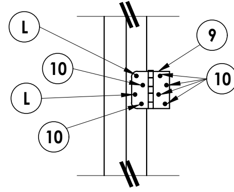
HINGE DETAIL
