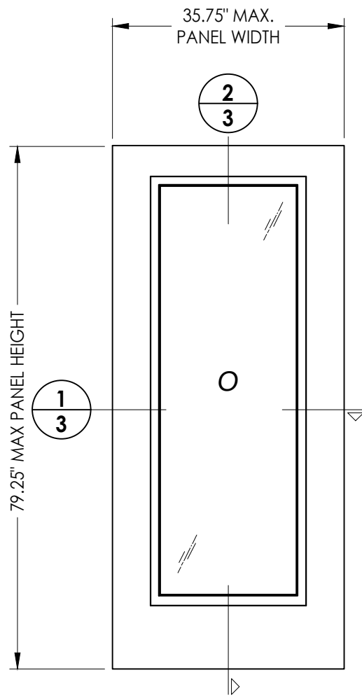
41 SIDELITE PANEL
