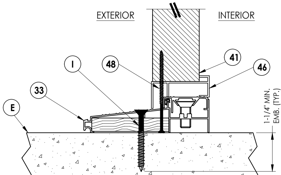
1 6 VERTICAL CROSS SECTION
