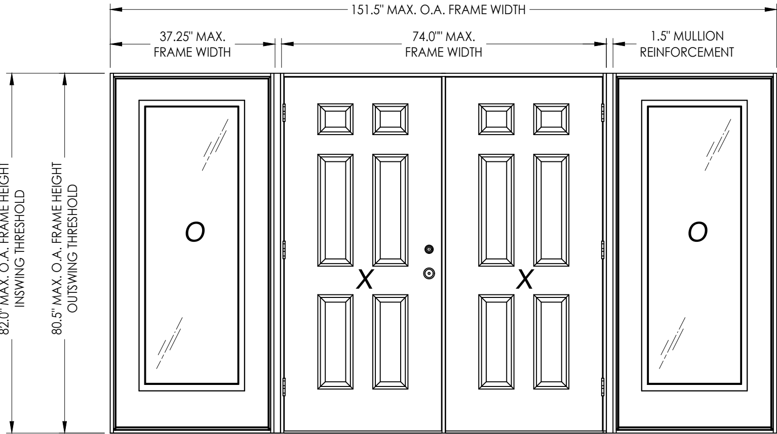
OPAQUE DOUBLE DOOR W/SIDELITES
