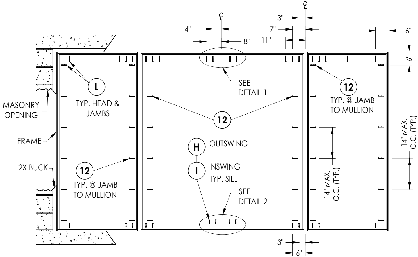
FRAME ANCHORING Masonry 2X buck construction
